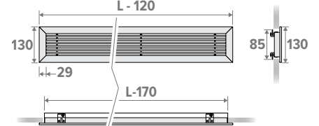
*minimum recess dimensions for mounting the grille
