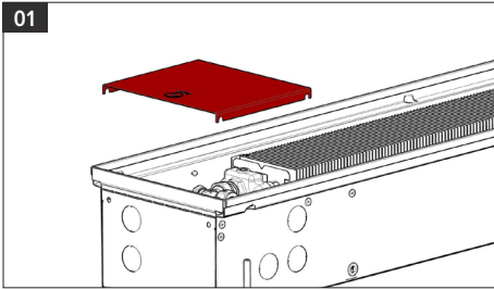
Remove the valve cover plate before installing the device.
